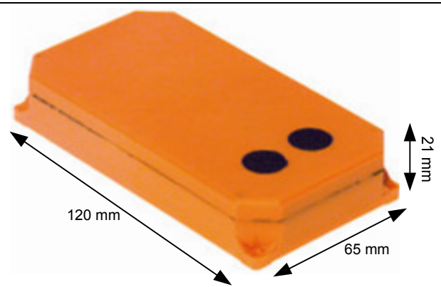
OIR-810
